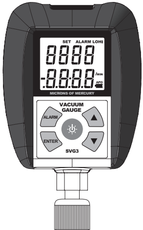
Vacuum Gauge
